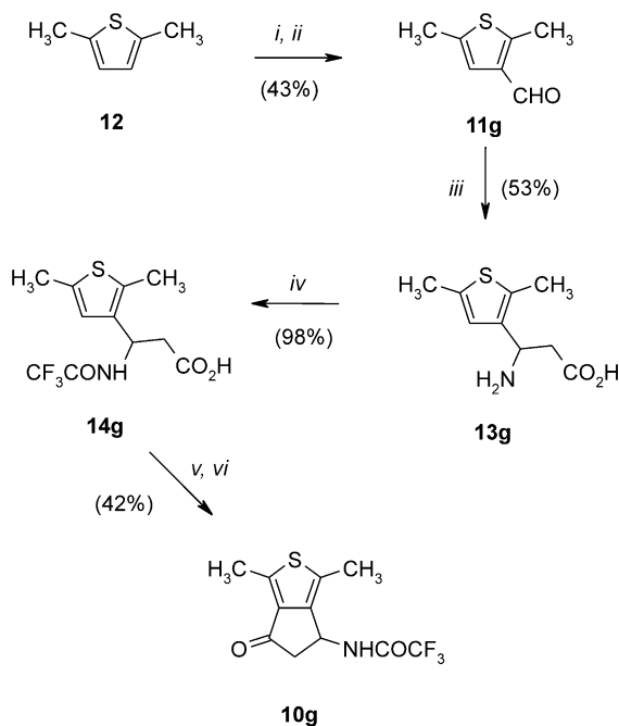
Scheme 1. Reagents: (i) POCl 3 , DMF (rt/30 min, 80 °C/3 h); (ii) NaOH, H 2 O (10 °C); (iii) CH 2 (CO 2 H) 2 , AcONH 4 , EtOH (refl/24 h); (iv) TFA 2 O, Et 2 O (rt/30 min); (v) SOCl 2 (refl/30 min); (vi) AlCl 3 , CH 2 Cl 2 (refl/2 h).
