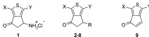
Figure 1. Structures of the 6-substituted cyclopenta[ c ]thiophenones 1–8 and cyclopentenones 9 .
