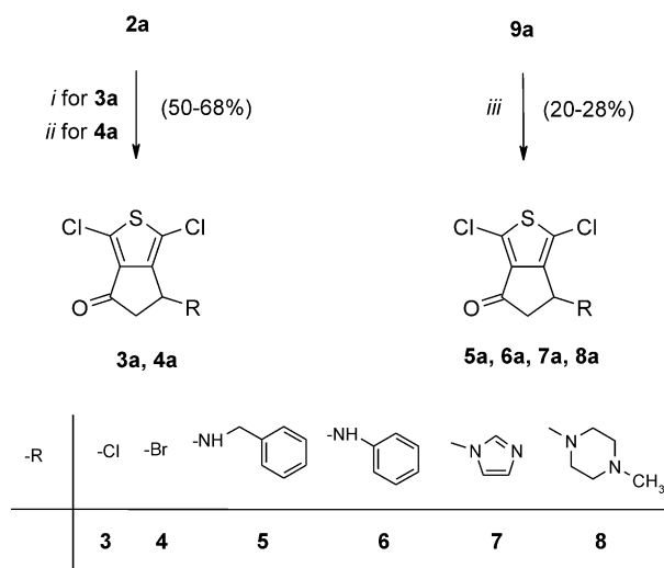
Scheme 3. Reagents: (i) SOCl 2 (refl/15 min); (ii) Br 2 , AcOH (rt/5 h); (iii) RH, CHCl 3 (refl/3 h).
