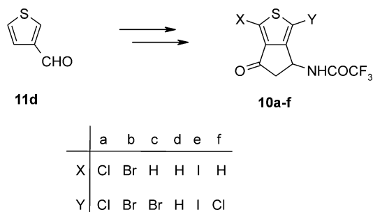
Figure 2. Synthetic route to 6-trifluoroacetylthio-5,6-dihydro-4H-cyclopenta[c]thiophen-4-ones 10a-f .
