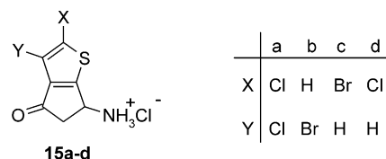
Scheme 3. Reagents: (i) SOCl 2 (refl/15 min); (ii) Br 2 , AcOH (rt/5 h); (iii) RH, CHCl 3 (refl/3 h).
