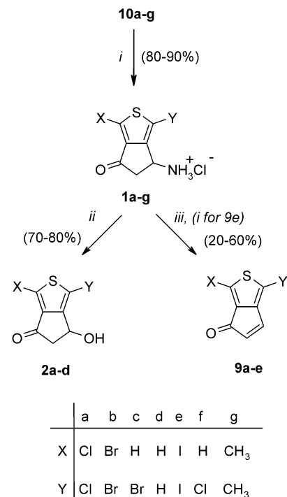
Scheme 2. Reagents: (i) HCl, H 2 O (refl, 12 h); (ii) NaNO 2 , AcOH, H 2 O (rt/4 h); (iii) NaNO 2 , TFA, H 2 O (rt/5 h).
